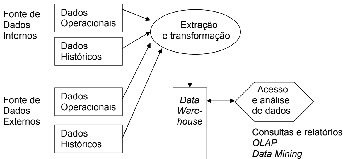
Figura 5: Data Warehouse e Data Mining.
